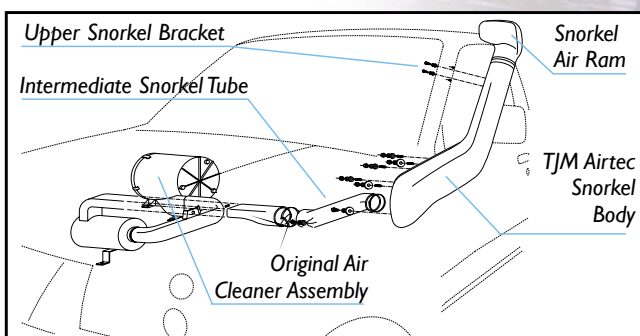
10/01+ DIESEL MODEL SHOWN - ILLUSTRATED ( LHS )
